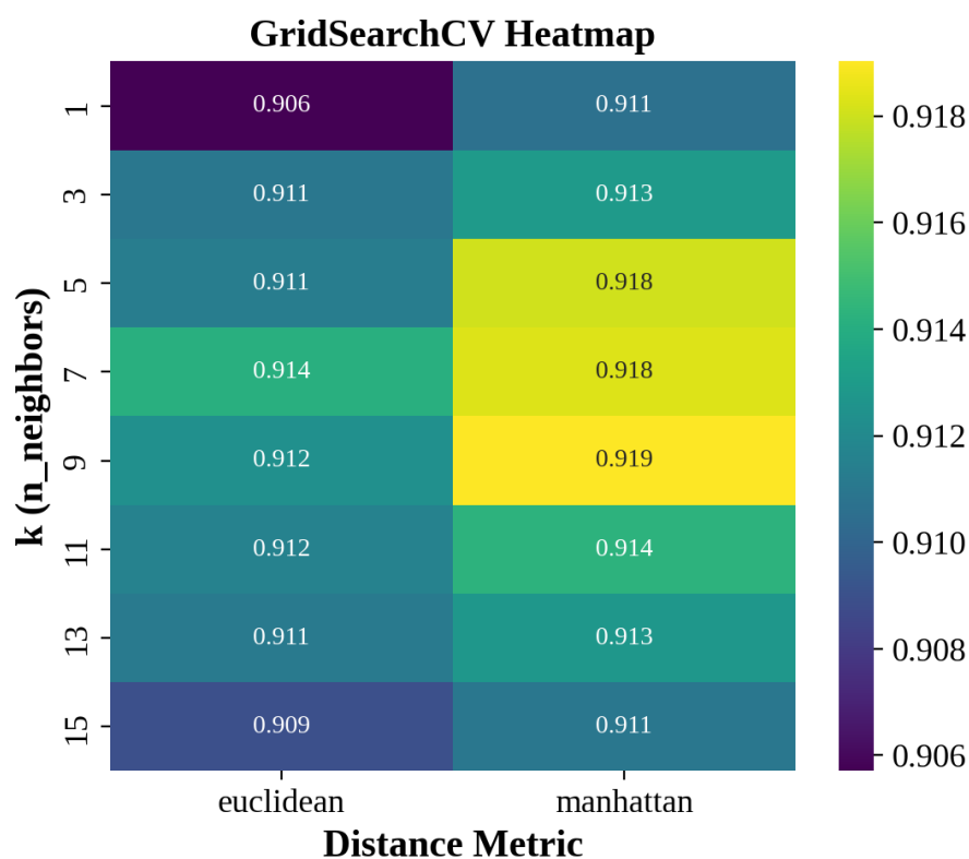
Figure 3: GridSearchCV mean CV accuracy across k and distance metric.
